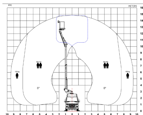
Working envelope
