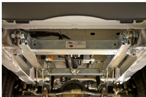
Hydraulic axle locking system
